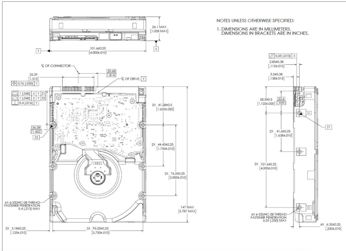
Figure 2-1. Mounting Dimensions
