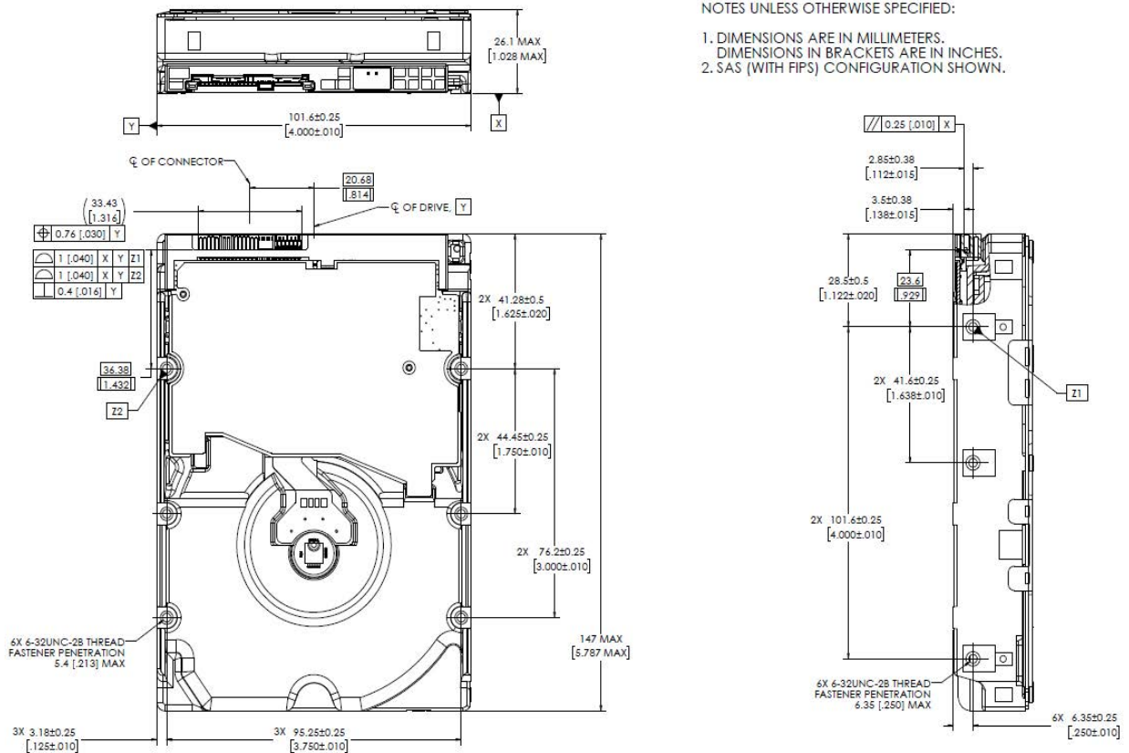
Figure 2-1. Mounting Dimensions
